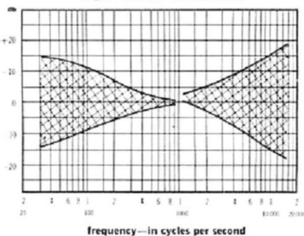
range of bass and treble controls
