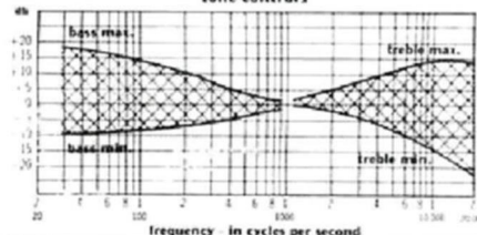
A340A amplifier relative frequency response
