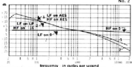
A440A preamplifier—phono equalizer curves No. 2
