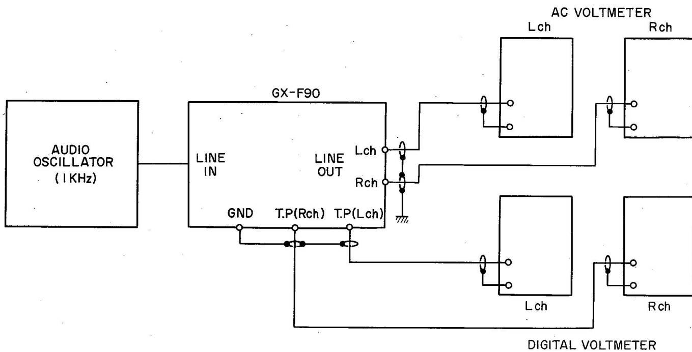
Fig. 28 Instrument Connection
