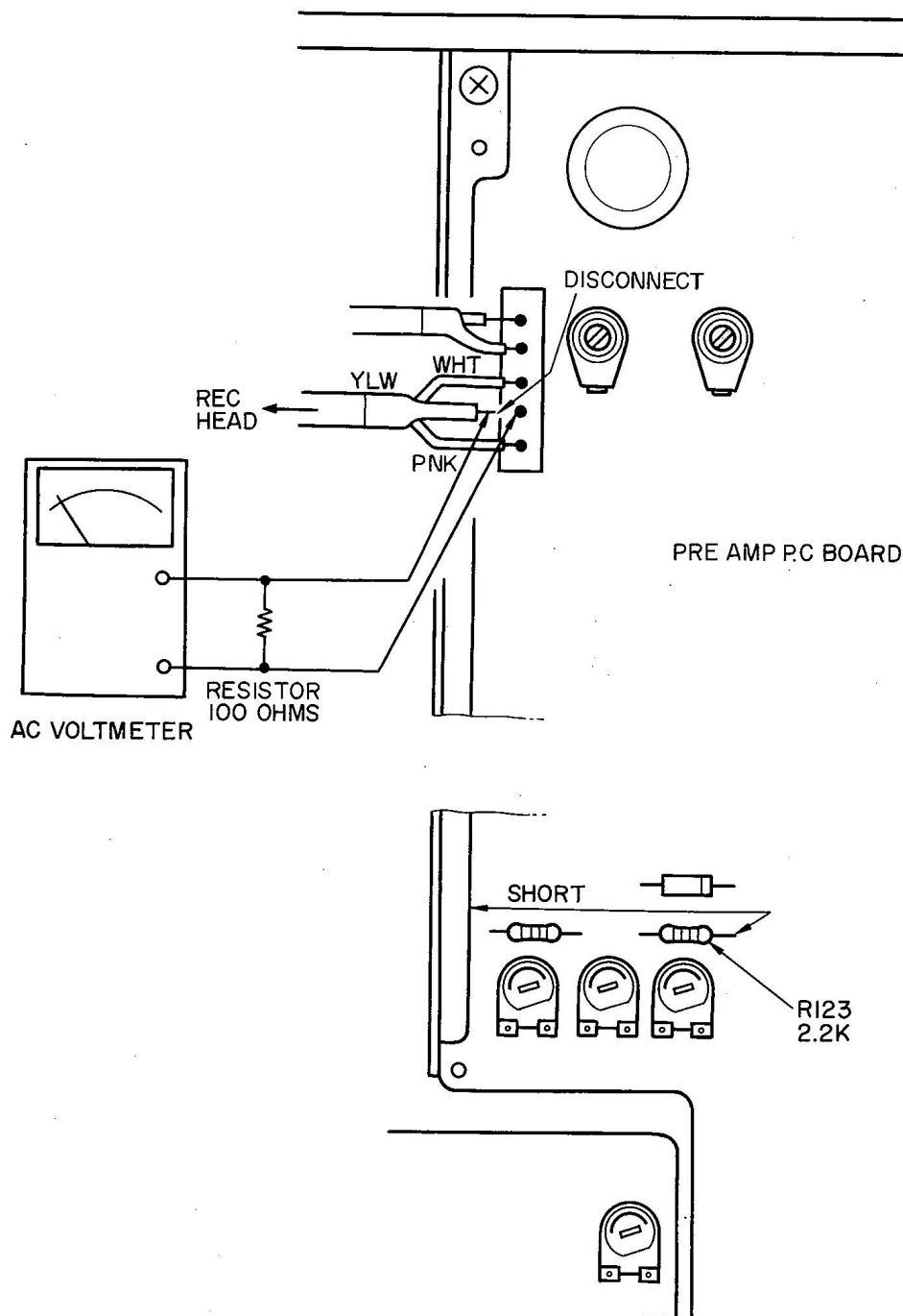
Fig. 26 Rec Peaking Adjustment
