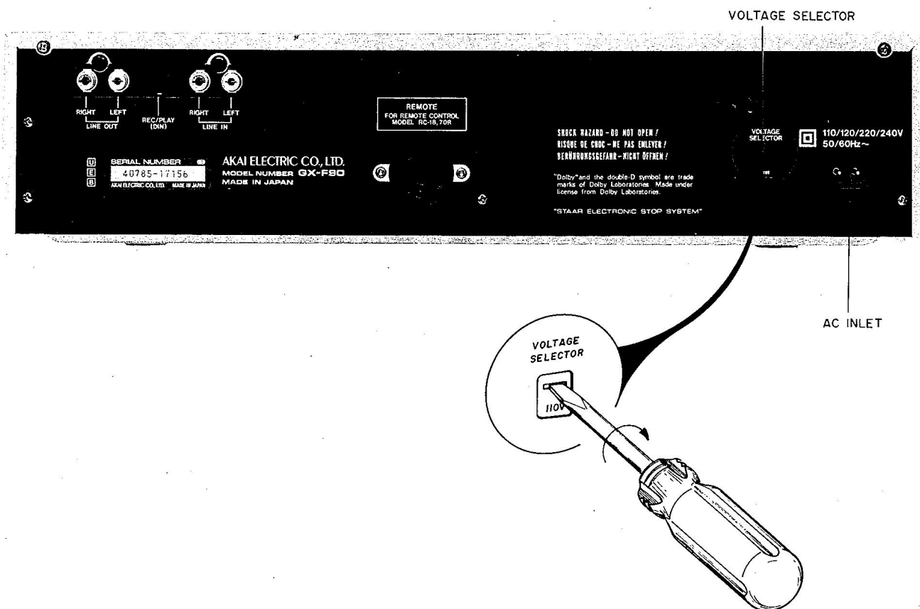
Fig. 4 Rear View (U/T, CEE, UK Models)
