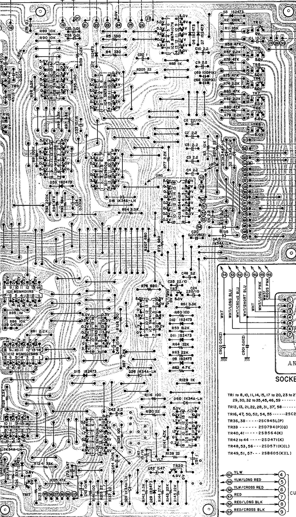
SYS.CON P.C BOARD CU-5032A
