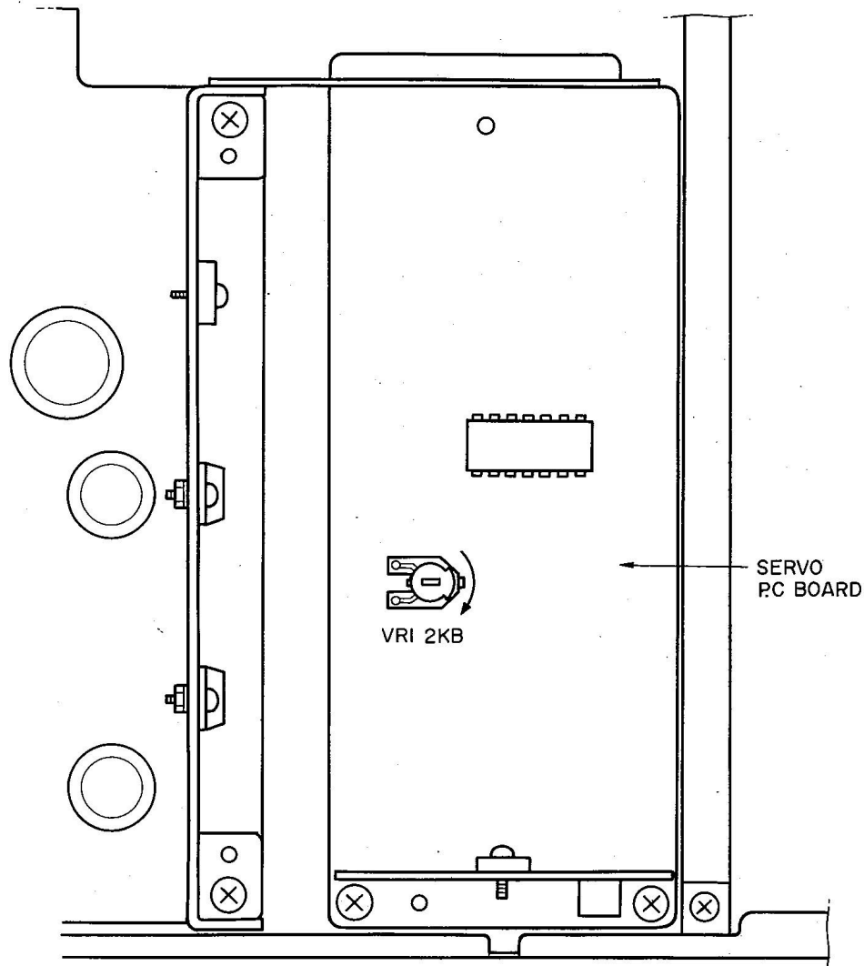
Fig. 20 Tape Speed Adjustment
