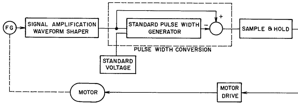
Fig. 14 Servo Circuit Block Diagram
