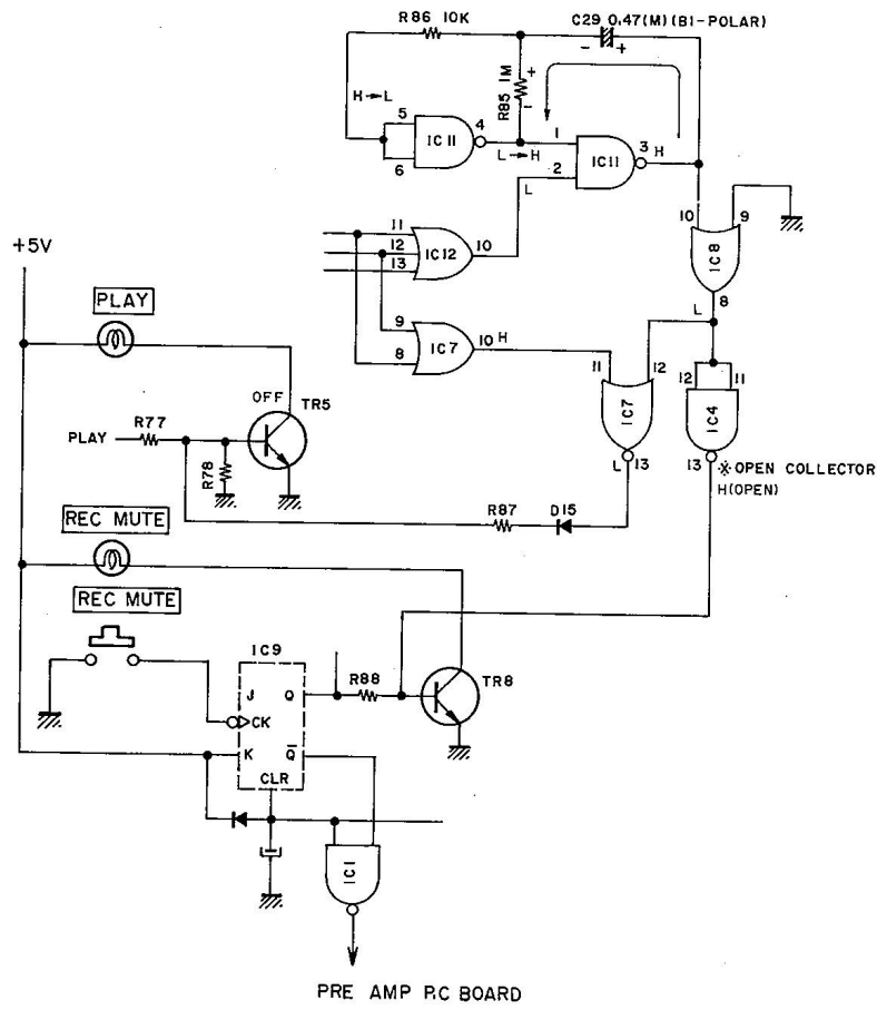
Fig. 7 Oscillation stopped
