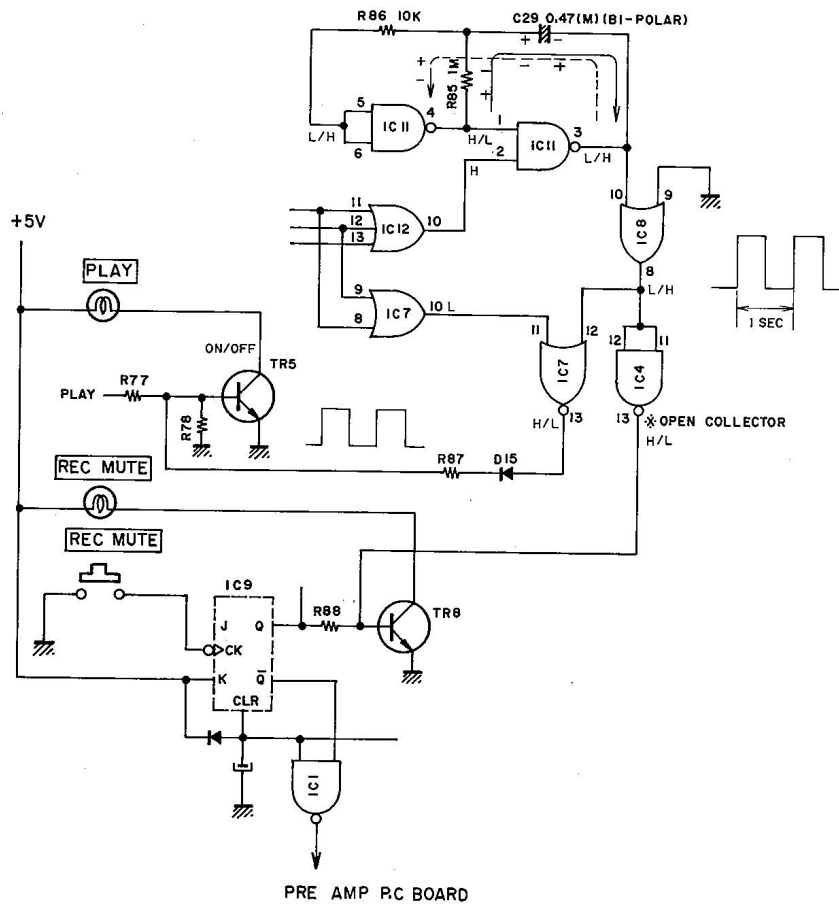
Fig. 8 Oscillation
