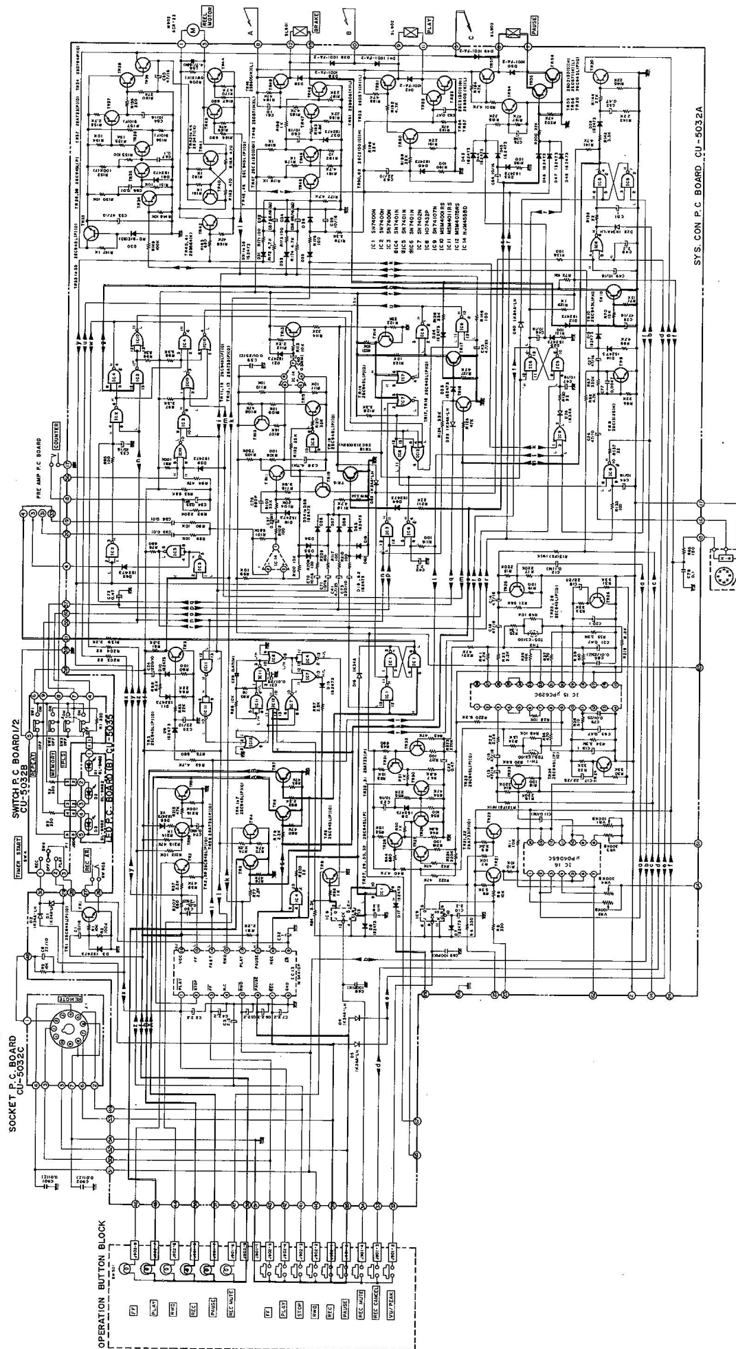
Schematic-4 REC/PAUSE MODE
