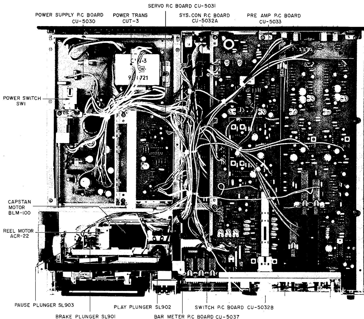
Fig. 3 Top View
