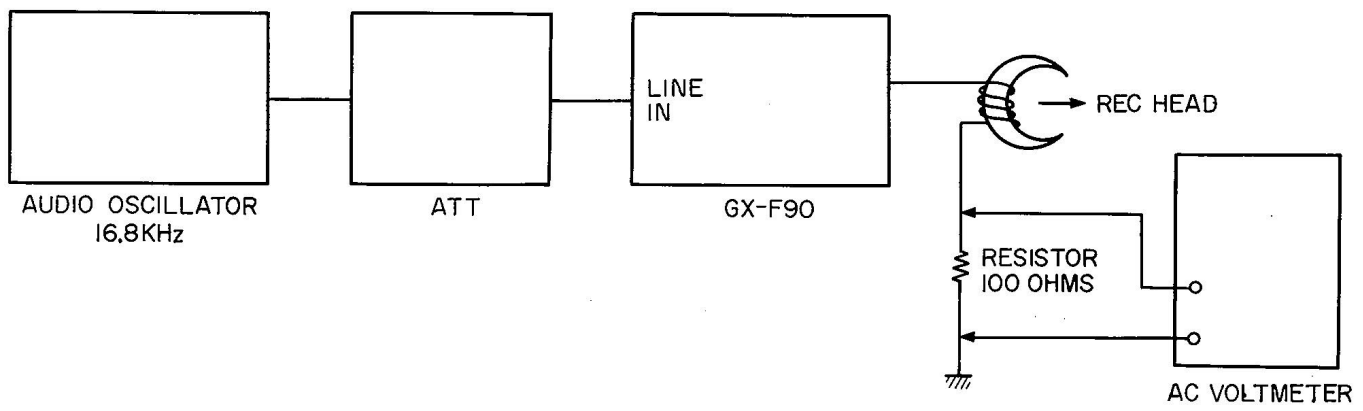
Fig. 25 Instruments Connection
