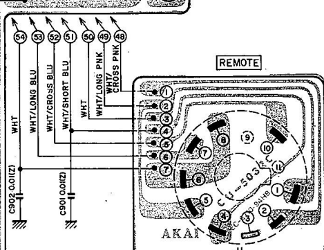
SOCKET P.C BOARD CU-5032C
