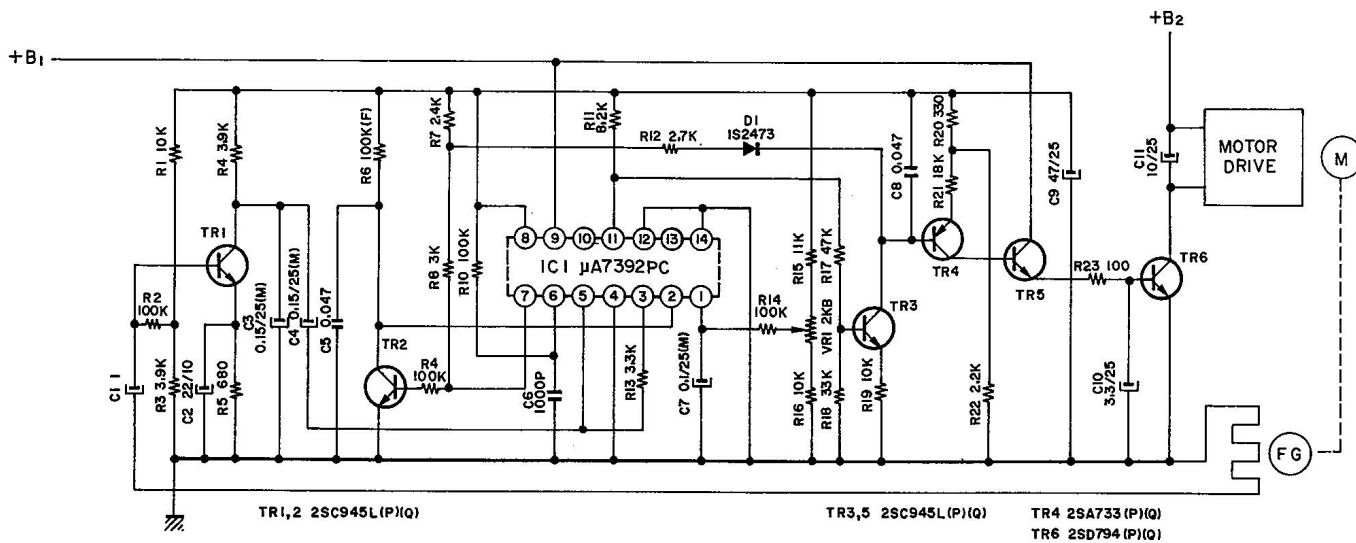
Fig. 15 Servo Circuit
