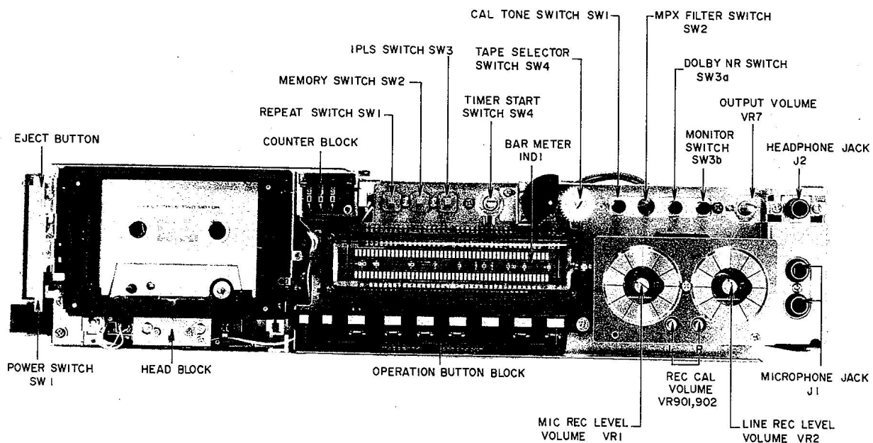
Fig. 2 Front View
