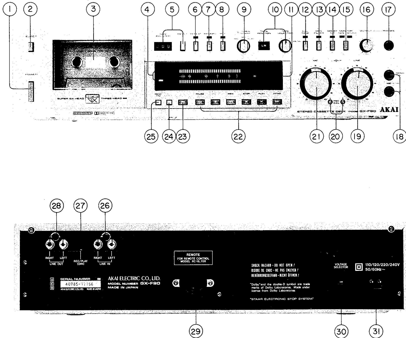
Fig. 1 Controls
