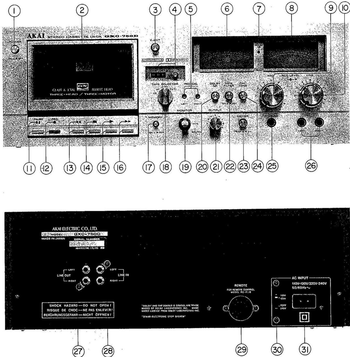
Fig. 1 Controls
