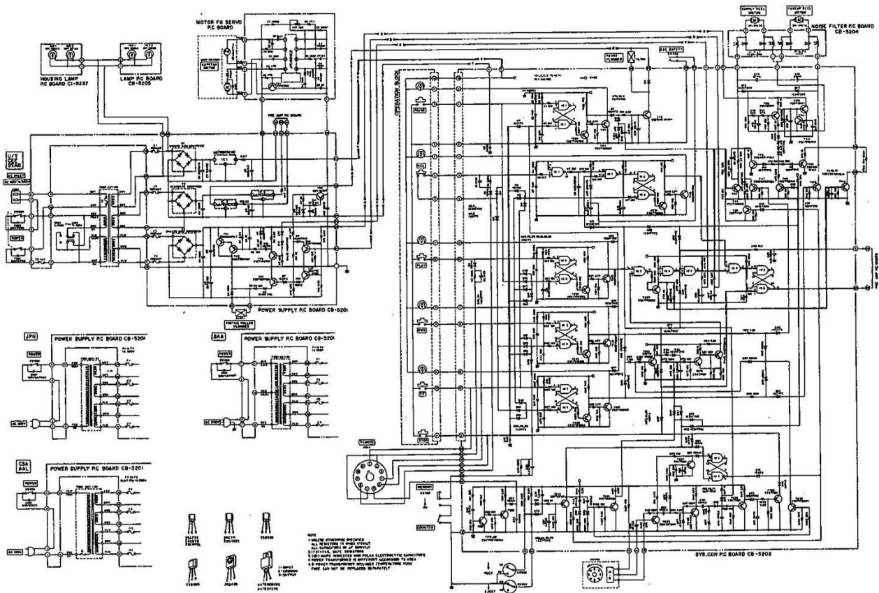
Schematic-2 STOP MODE
