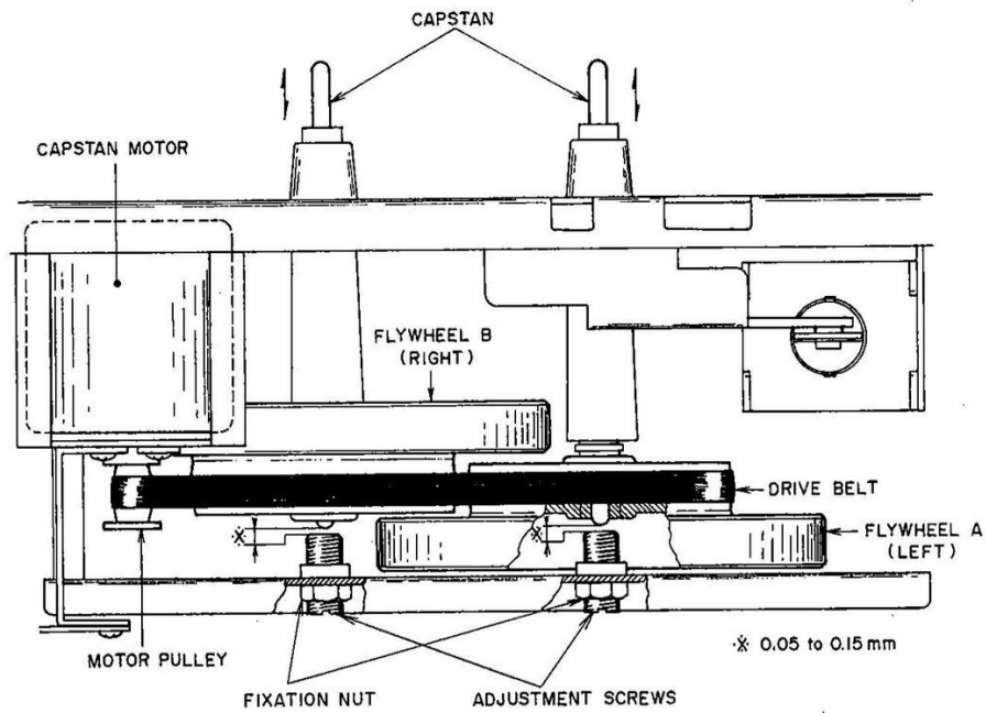
Fig. 4 Flywheel Thrust Loose Play Adjustment
