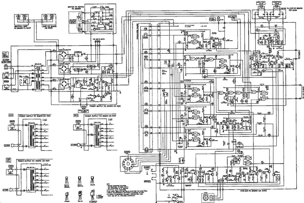
Schematic-3 PLAY MODE
