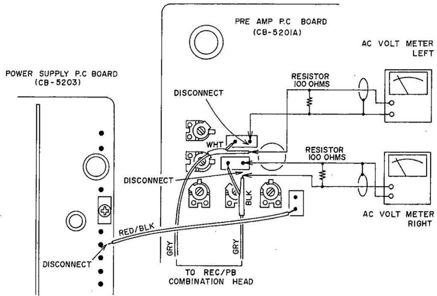
Fig. 16 Rec Peaking Adjustment
