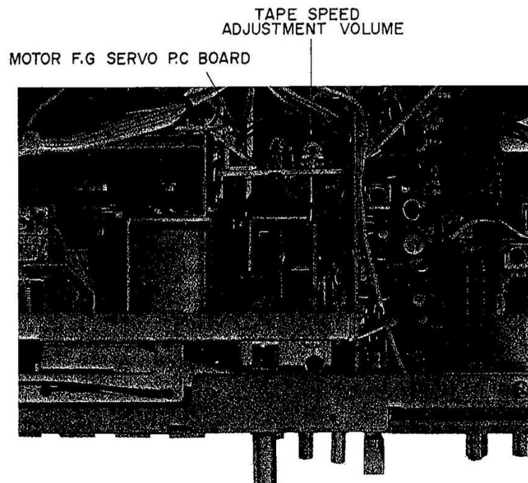
Fig. 10 Tape Speed Adjustment
