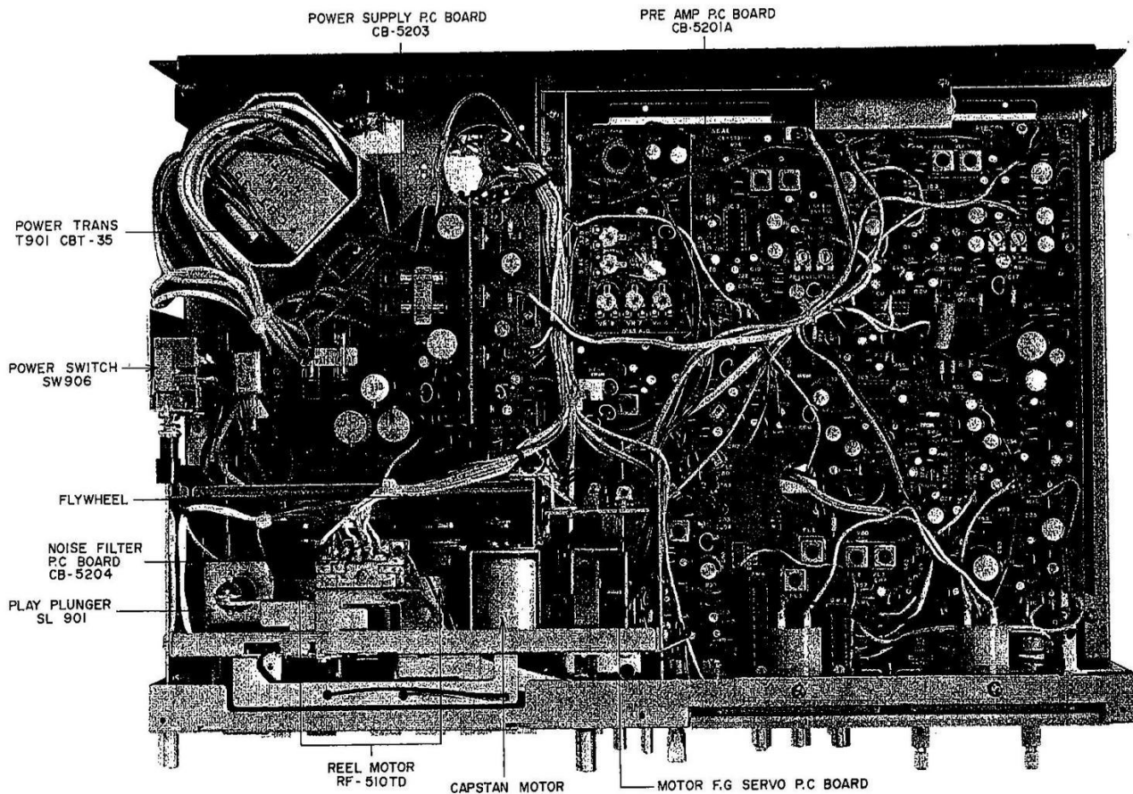
Fig. 3 Top View
