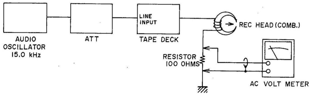
Fig. 15 Instruments Connections
