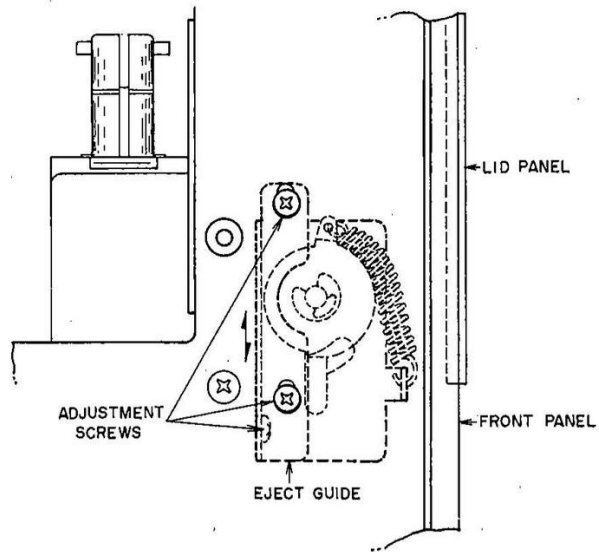
Fig. 9 Left Side of the Deck
