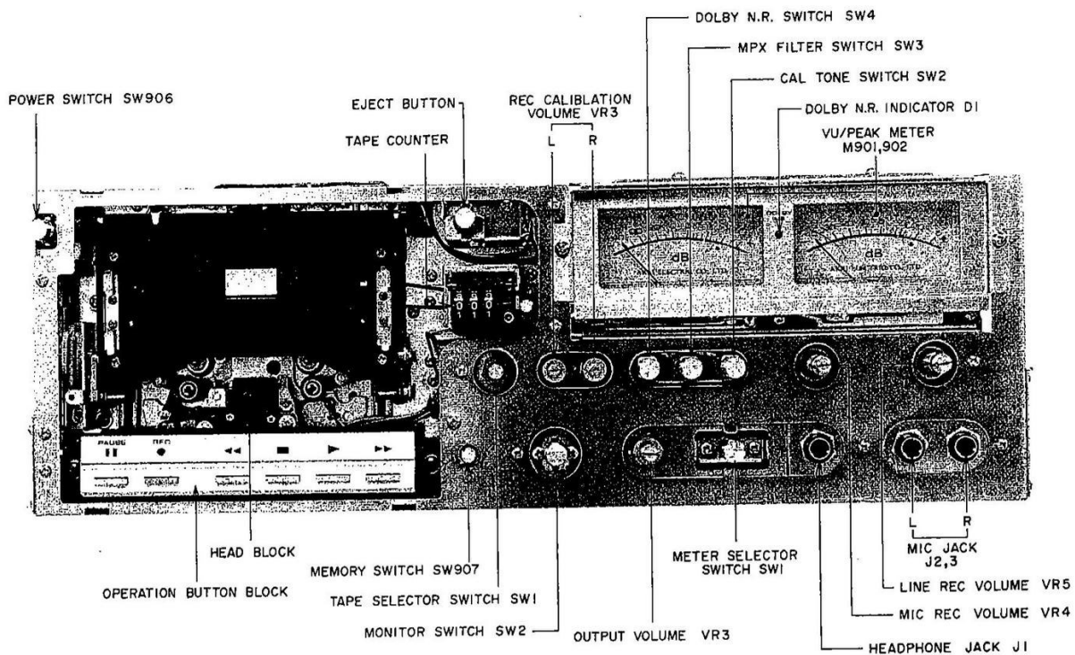
Fig. 2 Front View
