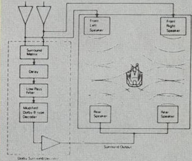
[Dolby Surround Decoder Block Diagram]
