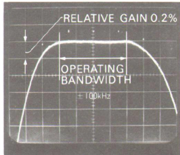
Fig.2 Differential Gain Characteristics of the Discriminator.
