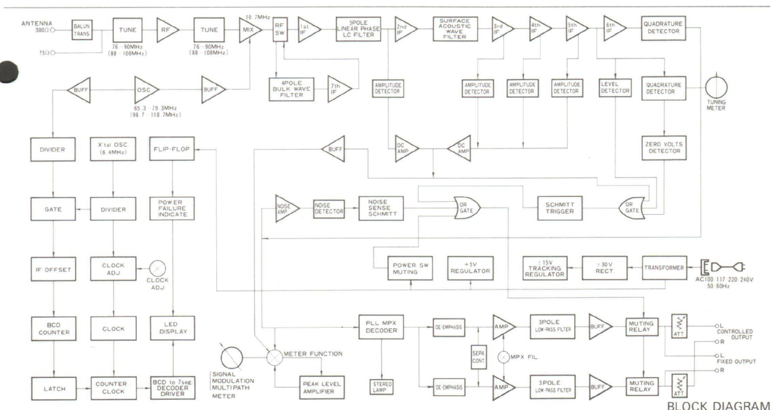
BLOCK DIAGRAM
