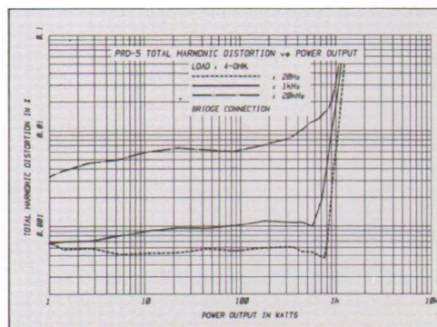
Total Harmonic distortion vs. Power Output Load: 4 ohms
