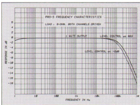
Frequency Characteristics Load: 8 ohms, Both channels driven
