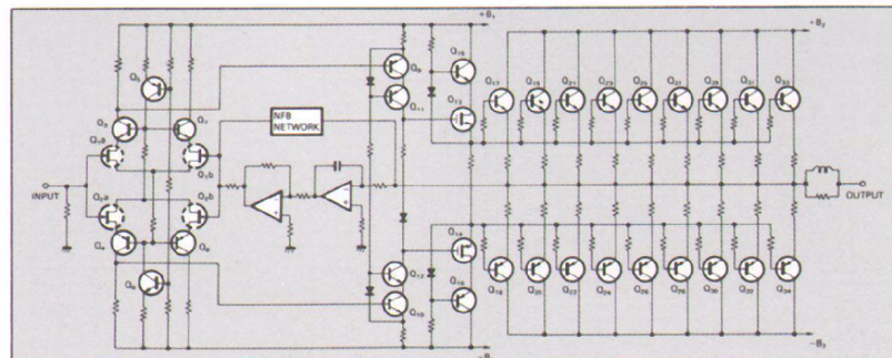
Fig. 1 PRO-5 Circuit Diagram
