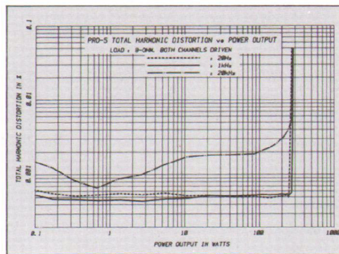
Total Harmonic distortion vs. Power Output Load: 8 ohms, Both channels driven
