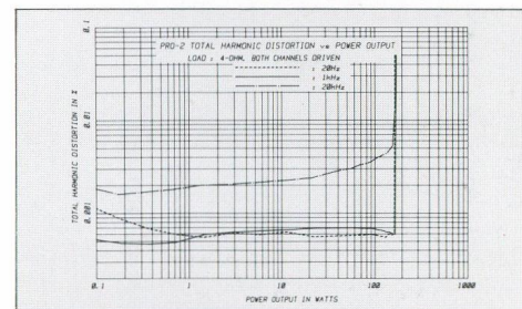
Total Harmonic Distortion vs. Power Output Load: 4 ohms, Both channels driven
