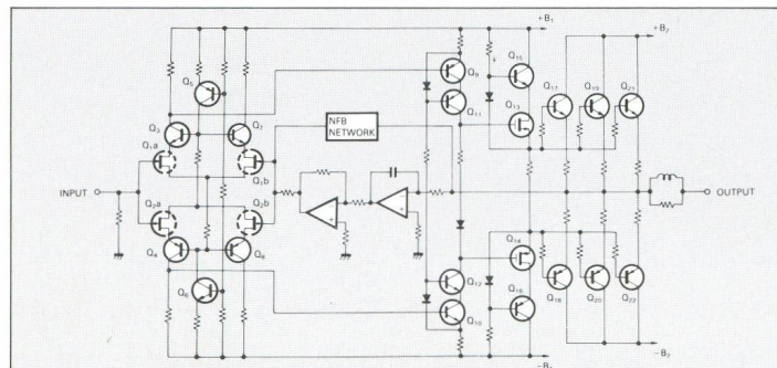
Fig. 1 PRO-2 Circuit Diagram
