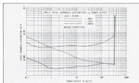
Total Harmonic Distortion vs. Power Output Load: 8 ohms, Bridge connection
