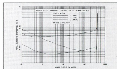
Total Harmonic Distortion vs. Power Output Load: 4 ohms, Bridge connection
