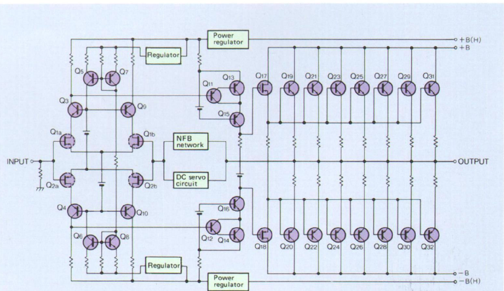
Fig. 1 P-600 Circuit Diagram
