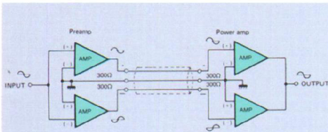
Fig. 3 Principle of the Balanced Type Network
