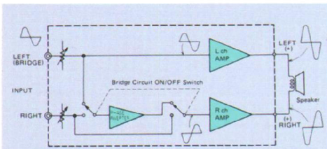
Fig. 2 Principle of the Bridging Connection
