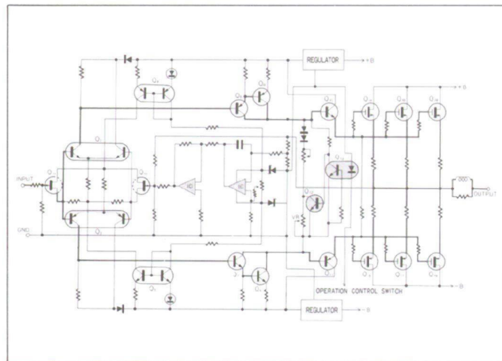
Fig. 1 MOS FETs' SYMMETRICAL PUSH-PULL DC POWER AMP.
