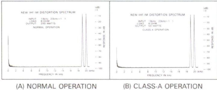
Fig. 2 NEW IHF-IM DISTORTION SPECTRUM
