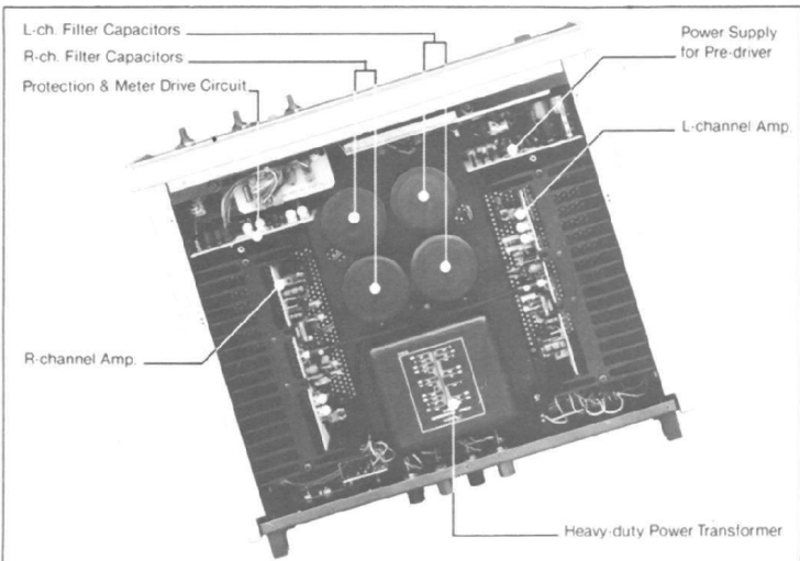
Internal View
