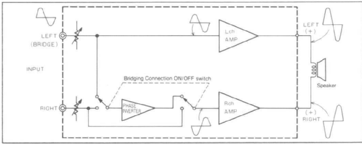
Schematic diagram of Bridging Connection
