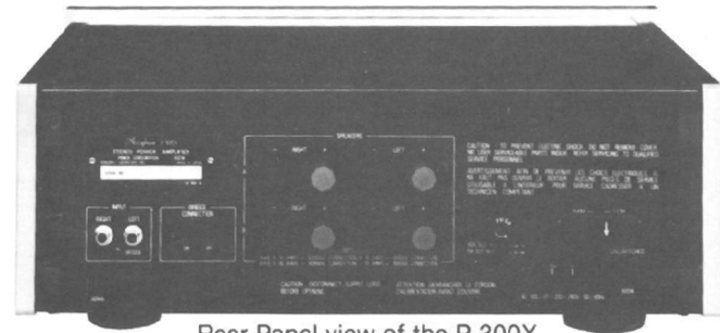
Rear Panel view of the P-300X
