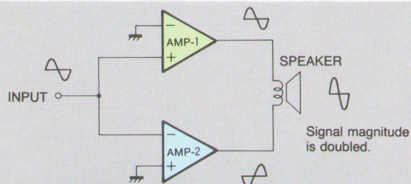
Fig. 2 Operating Principle of Bridge Connection
