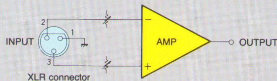
Fig. 5 Balanced Input Circuit
