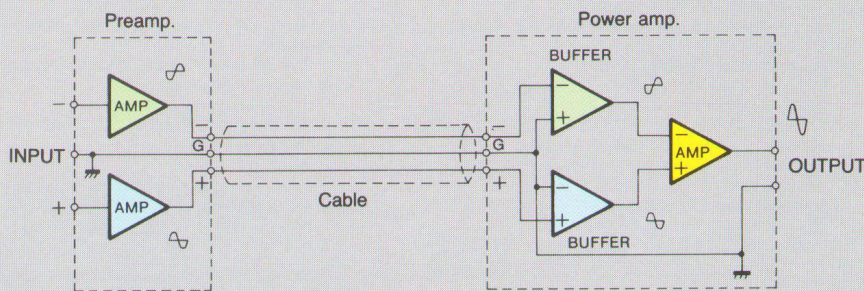
Fig. 4 Operating Principle of Balanced Network
