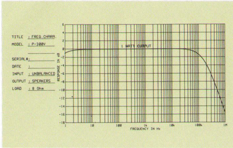
● FREQUENCY CHARACTERISTIC
