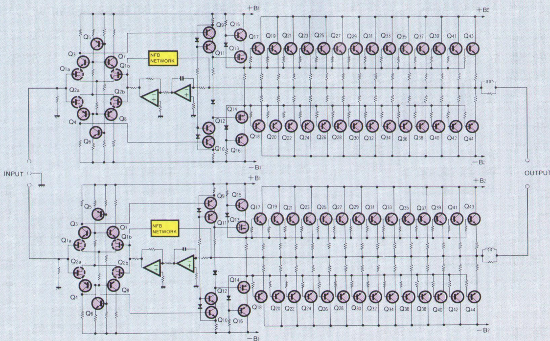
Fig. 2 Block Diagram of M-1000
