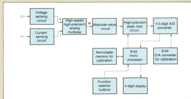
Fig. 2 Block diagram of M-1000 digital power meter
