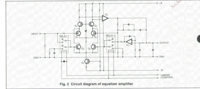
Fig. 2 Circuit diagram of equalizer amplifier
