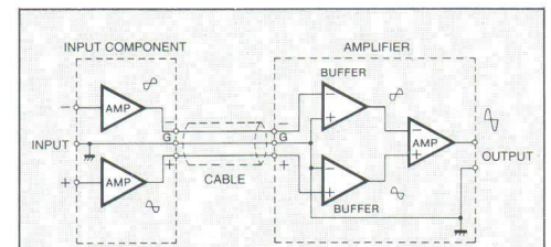
Fig. 4 Principle of the balanced output/input connection
