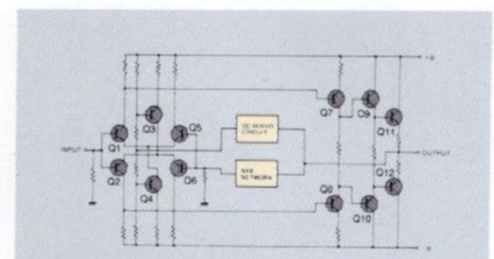
Fig. 3 Circuit Diagram of Head Amplifier
