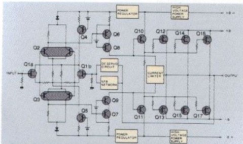
Fig. 1 Circuit Diagram of Power Amplifier
