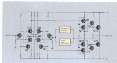
Fig. 2 Circuit Diagram of Equalizer Amplifier
