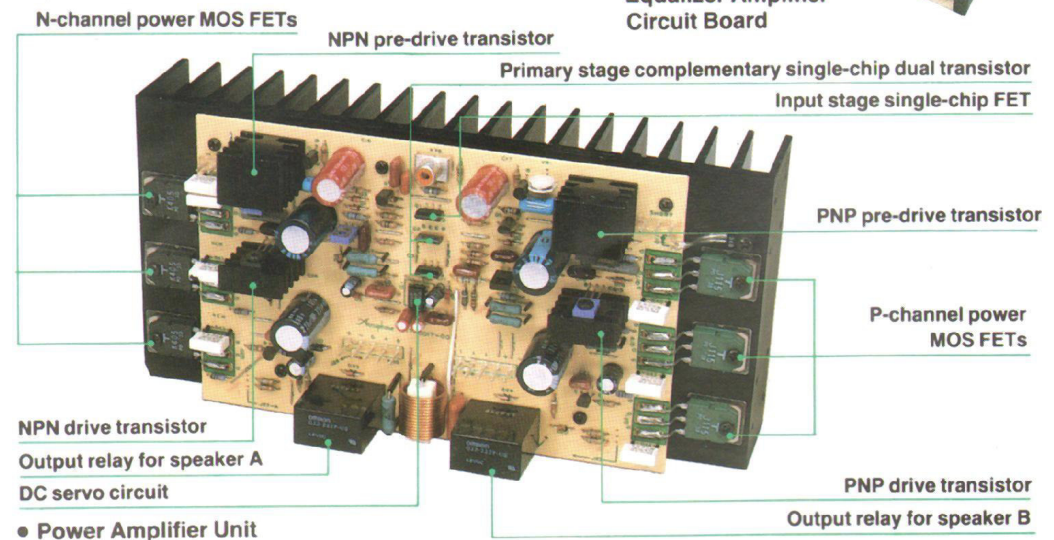
• Head Amplifier/Equalizer Amplifier Circuit Board
