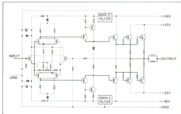
(FIG. 1) MOS FETs' SYMMETRICAL PUSH-PULL POWER AMP.
