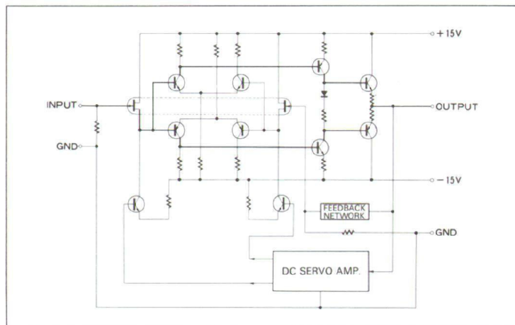
(FIG. 2) SERVO CONTROLLED HIGH-LEVEL AMP.
