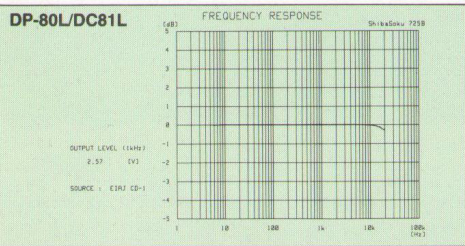
• Frequency Characteristic
