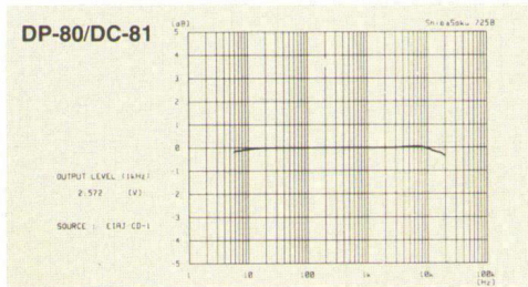
● Frequency Characteristic
