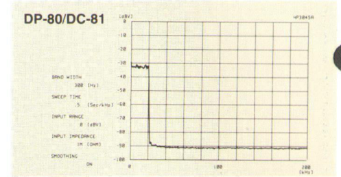
● Spectrum Analysis of -20dB White Noise
