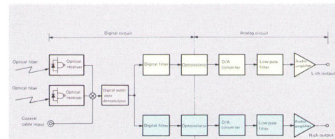
Fig. 6 DC-81 Block Diagram
