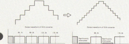
Fig. 4 Operational Concept of Digital Oversampling Filter
