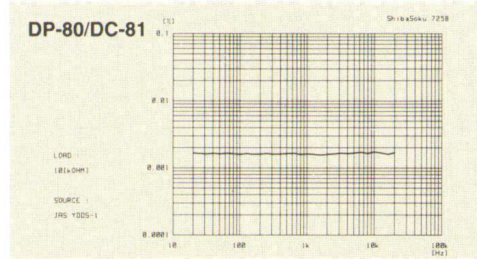
● THD + Noise vs. Frequency Characteristic
