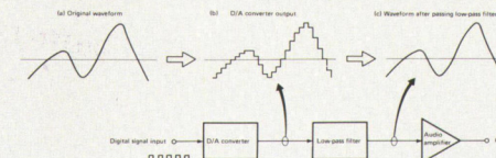
Fig. 1 Configuration of Typical CD Player
