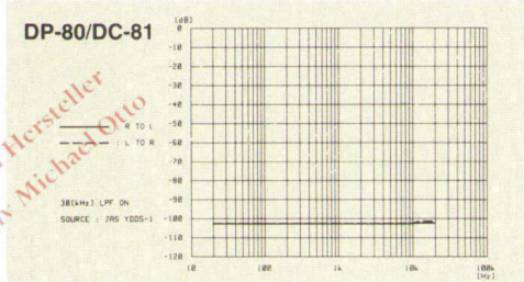
● Channel Separation Characteristic
