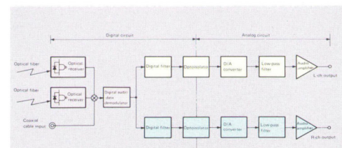
Fig. 6 DC-81 Block Diagram
