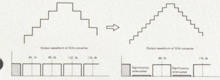
Fig. 4 Operational Concept of Digital Oversampling Filter
