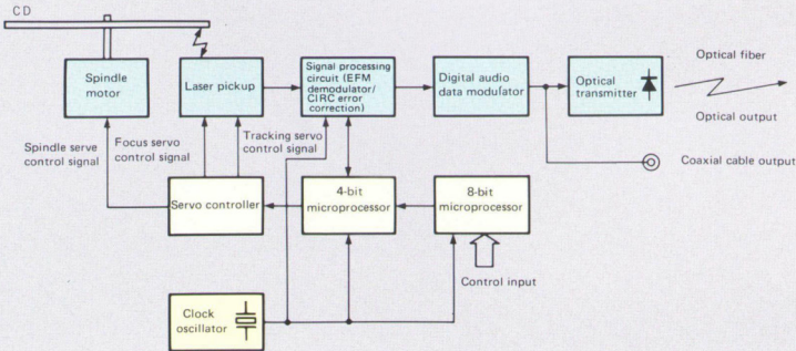
Fig. 5 DP-80 Block Diagram
