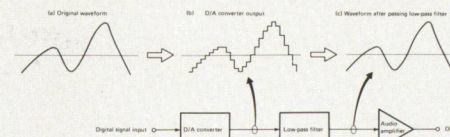
Fig. 1 Configuration of Typical CD Player
