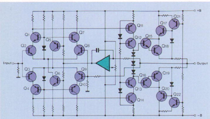
Fig. 4 Circuit Diagram of the Head Amplifier
