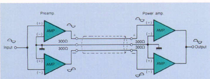
Fig. 5 Principle of the Balanced Type Network
