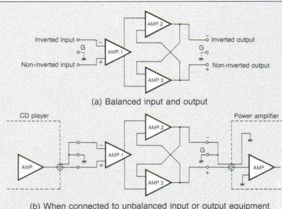
Fig. 2 Balanced line amplifier stage
