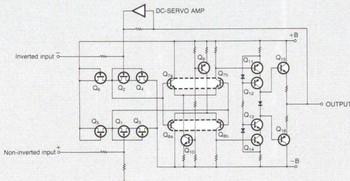
Fig. 3 Circuit diagram for the balanced input amplifier
