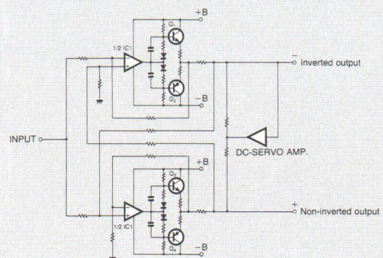
Fig. 4 Circuit diagram for the balanced output amplifier
