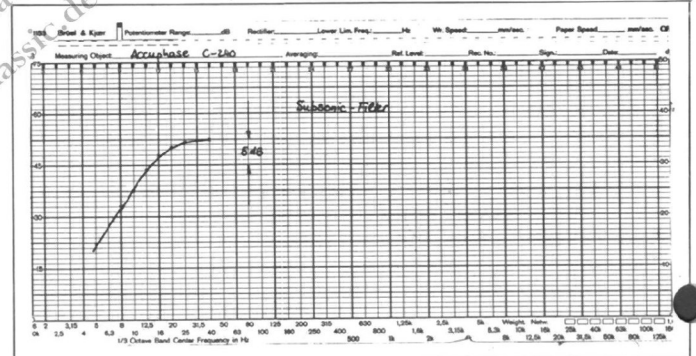
Subsonic-Filter
