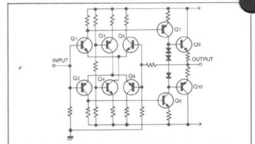
Circuit Diagram of the Head Amplifier
