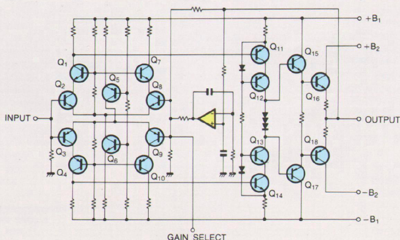
Fig. 3 Circuit Diagram of the Head Amplifier
