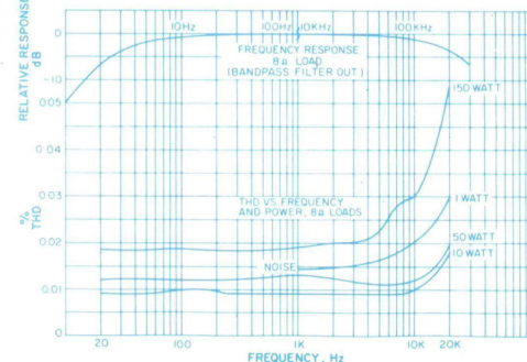
Fig. 13—Relative response at one-watt output (top), distortion vs. power and frequency (bottom).
