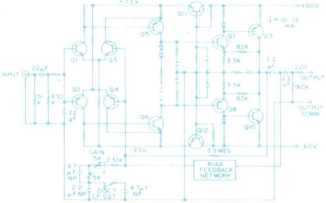
Fig. 6—Phono preamp circuit, showing simplified version of Disc 1, 2 LF enhance circuit.
