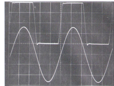
Fig. 14—20 kHz (top) square-wave response of power amplifier, 8 ohms, 200 watts. 20 kHz (bottom) sine wave response, 1 μF load, 40 volts RMS.
