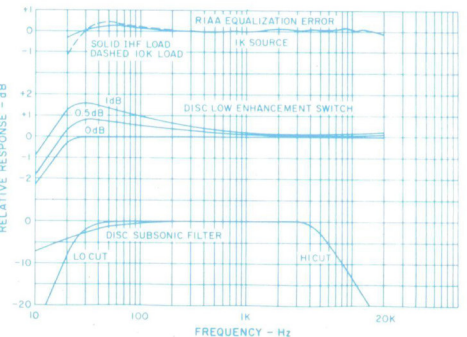
Fig. 7—Phono preamp response curves, including subsonic filter and 3-position LF enhancement switch.
