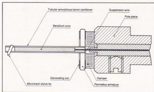
Fig. 1 Cross Section of Moving Element
