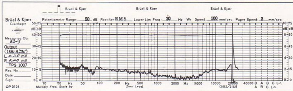
Fig. 2 Frequency Response & Crosstalk
