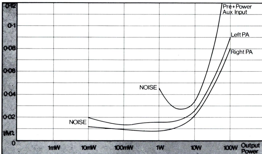
Fig. 14. Intermodulation distortion for the E202
