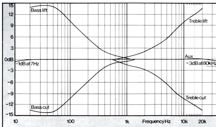
Fig. 12. Preamp response and tone controls
