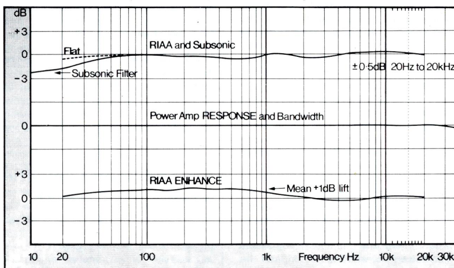
Fig. 11. Power amplifier response, -20dB and half power bandwidth
