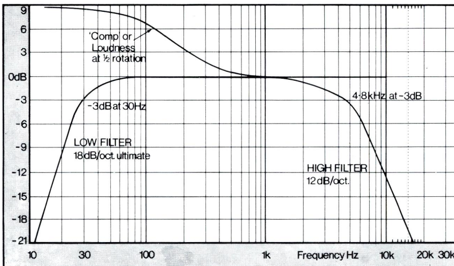
Fig. 13. Preamp filter and loudness responses
