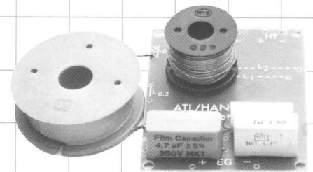
Frequenzweiche Type HD 308i
