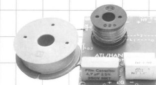
Frequenzweiche Type HD 308i
