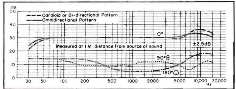
Guarantee frequency response curve
