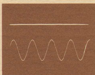
Sine Wave & Distortion Products 20 KHz 100 m Watt Scope: 20 µsec/cm Top: Distortion Products 0.2 v/cm Bottom: Output 1 v/cm
