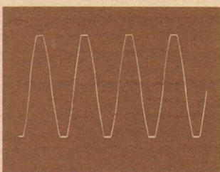
Clipping 2 KHz 190 Watts 8 Ohm Scope: 0.2 msec/cm 20 v/cm
