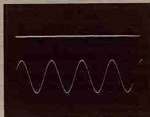
Sine Wave & Distortion Products 20 KHz 100 m Watt Scope: 20 \mu sec/cm Top: Input 0.2 v/cm Bottom: Output 1 v/cm
