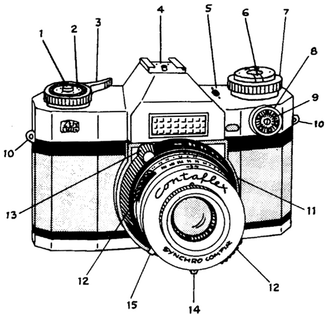
I-1.1. CONTAFLEX SUPER, FRONT VIEW
