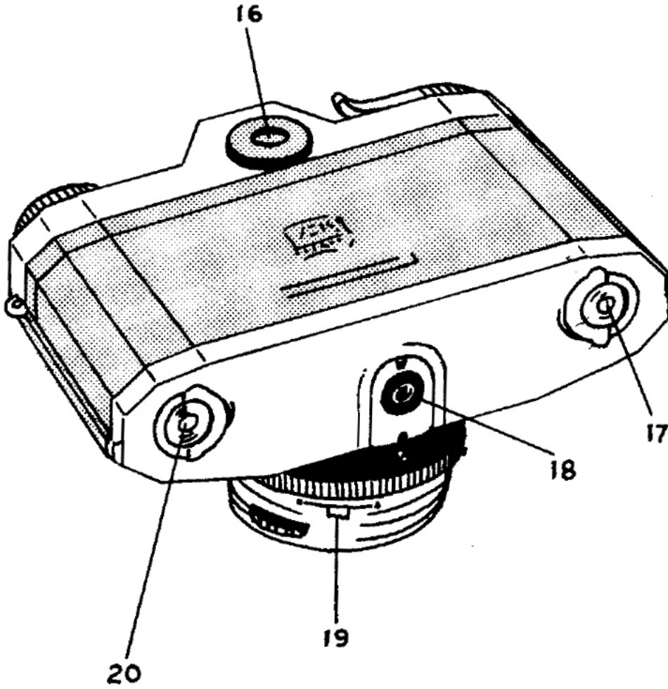
I-1.1. CONTAFLEX SUPER, BACK VIEW
