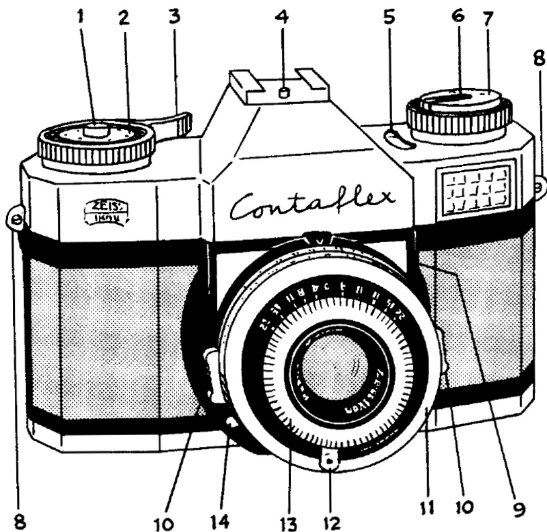
I-1.2. CONTAFLEX PRIMA, FRONT VIEW
