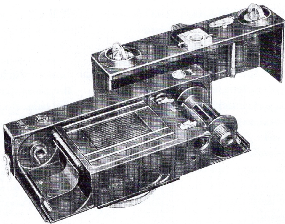
CONTAX opened, showing accessibility of interior
