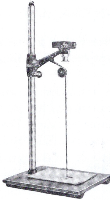
Large copying stand
