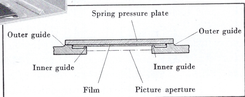
Back cover of CONTAX showing pressure plate
