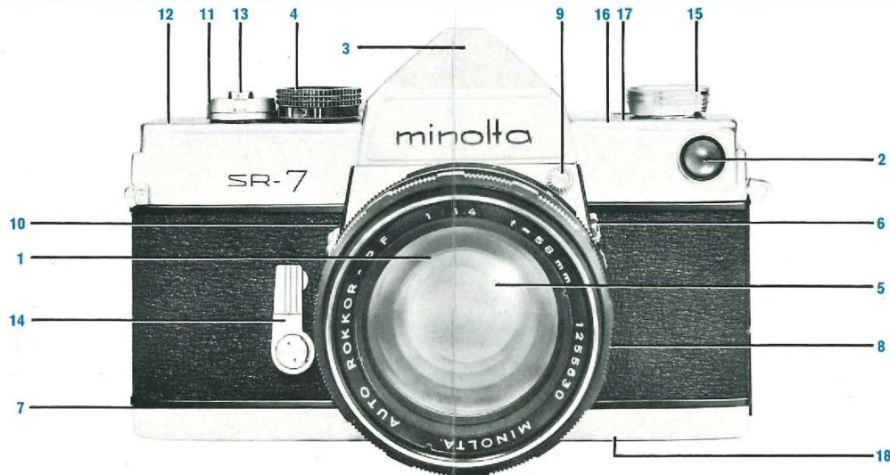
Minolta SR-7 with built-in CdS meter, speeds to 1/1000th second, microprism finder, mirror lock
