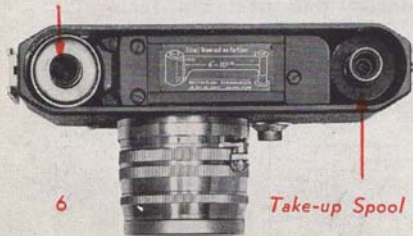
Canon Film Magazine
