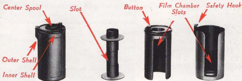
Assembled Film Magazine Center Spool Inner Shell Outer Shell
