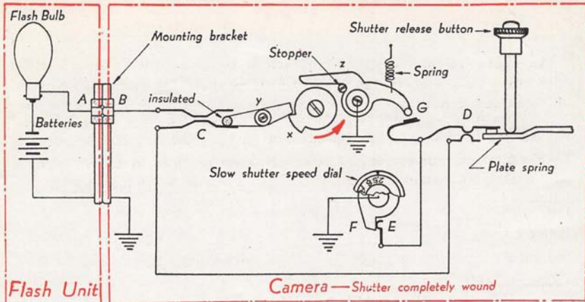
Schematic Diagram of Canon Model IV and IV-F BUILT-IN FLASH SYNCHRONIZER *
