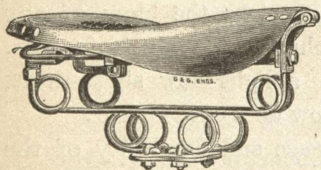
FIG. 25—VICTOR SAFETY SADDLE AND SPRING (DETACHABLE LEATHER).
