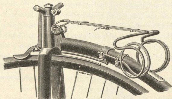
FIG. 20—VICTOR SWING SADDLE, WITH LEATHER OFF
