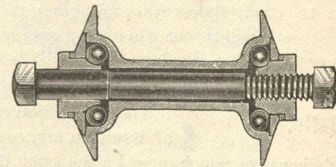
FIG. 6—SECTIONAL VIEW OF REAR HUB.
