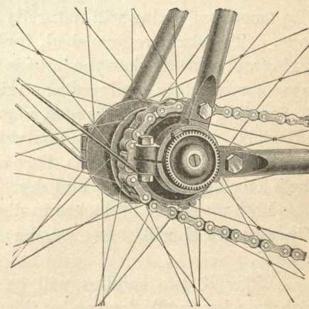
FIG. 24—SAFETY REAR HUB.
