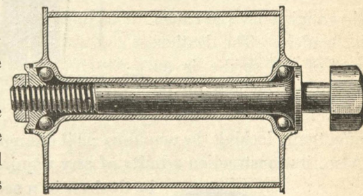
FIG. 18—SECTIONAL VIEW OF PEDAL, SHOWING BALL BEARINGS.
