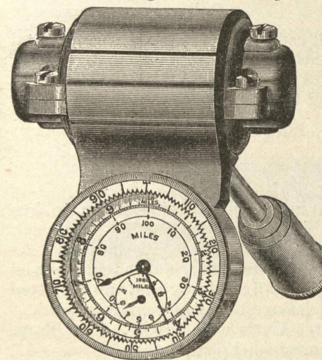
FIG. 32—VICTOR HUB CYCLOMETER.
