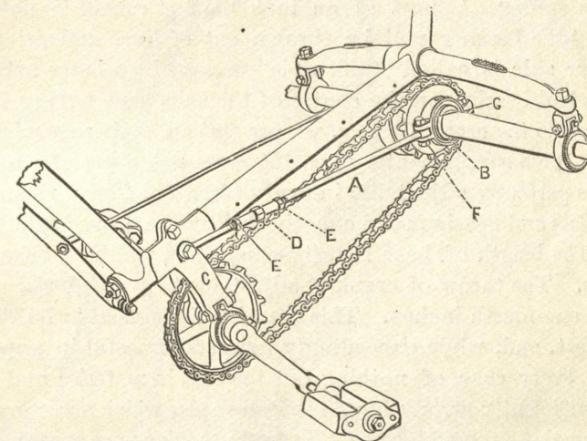
FIG. 29—SECTION OF TRICYCLE FRAME, SHOWING CONSTRUCTION OF INFLEXIBLE AXLE.
