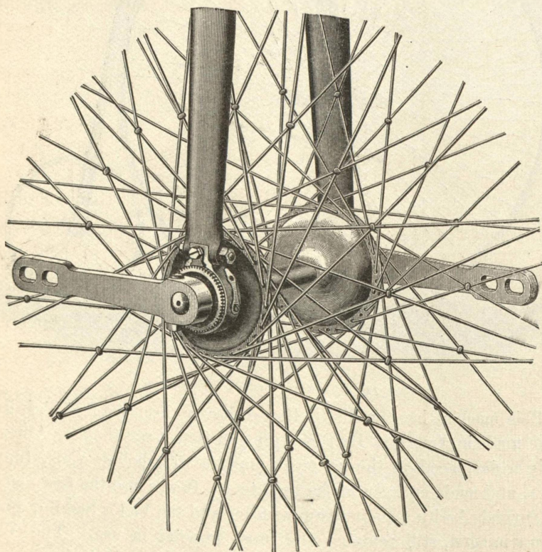
FIG. 15—SHOWING HUB, CRANK AND ARRANGEMENT OF SPOKES.
