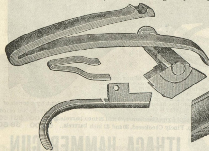
The above Cut represents all the Working Parts of the Lock of "The New Baker Gun"—Full Size.
