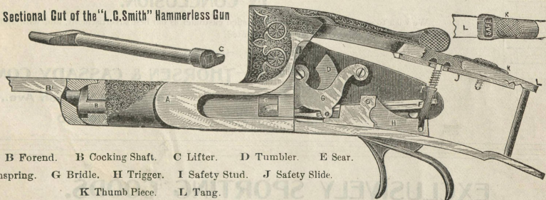
Sectional Cut of the "L. C. Smith" Hammerless Gun
