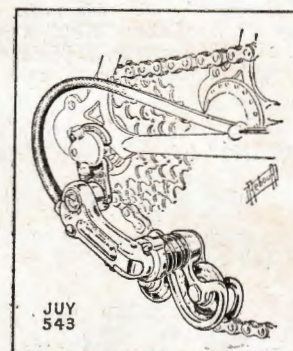
SIMPLEX "JUY 543" GEAR SELECTOR
