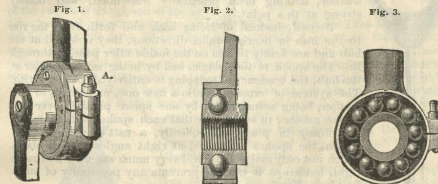
ADJUSTABLE PATENT FRONT BEARINGS.
