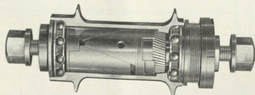
Sectional View Showing Arrangement of Parts.
