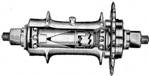
New HERCULES Coaster Brake.
