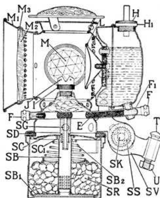
No. 3370—Solar Lamp Parts
