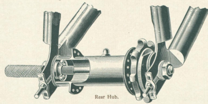
Rear Hub.
