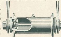
Front Hub.
