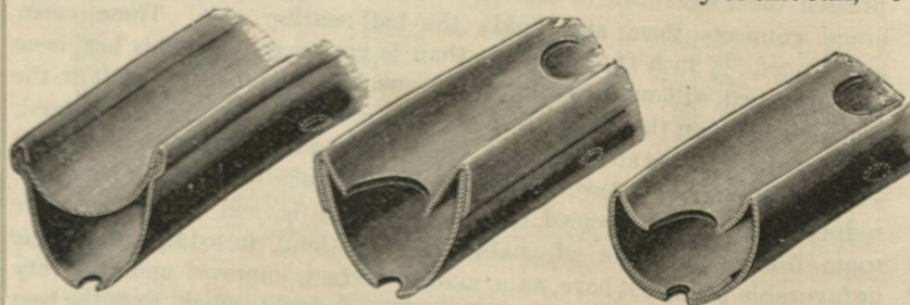
Rims of imported pattern used by other makes, weakened by unnecessary drilling to insert spokes and nipples.
